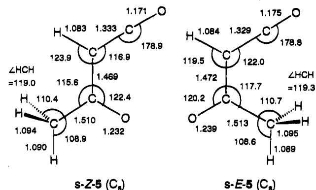
Figure 3. Optimized geometries (MP2/6-31G*) of s-Z and s-E -acetylketenes (bond lengths (Å) and bond angles (deg)).
