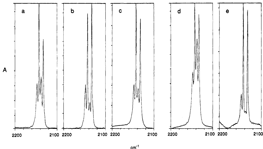
Figure 2. Partial FTIR spectra (Ar, 14 K) of s-Z/s-E -acetylketene ( 5 ) produced by FVP of precursors 1-4 : (a) from 1 at 400 °C; (b) from 3 at 400 °C; (c) from 4 at 600 °C; (d) from 3 at 400 °C with low argon/solute ratio (10 min deposition time); and (e) from 4 at 600 °C with high argon/solute ratio (45 min deposition time). Bands due to s-Z-5 at 2143 and 2148 \text{cm}^{-1} ; bands due to s-E-5 at 2133 and 2137 \text{cm}^{-1} . For discussion, see text. A full spectrum corresponding to Figure 2b is given in the supplementary material.
