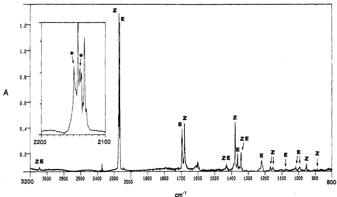
Figure 1. FTIR spectrum (Ar, 14 K) of s-Z/s-E -acetylketene ( 5 ) produced by FVP (400 °C, 10^{-5} mbar) of 2 . Assignments based on E/Z isomerization experiments (see Figures 4c and 5) and ab initio calculations (for exact values and discussion of individual bands, see Table 1). Weak bands at 2345 and ca. 1600 \text{cm}^{-1} are due to \text{CO}_2 and \text{H}_2\text{O} , respectively. The inset shows the expanded ketene region (2200–2100 \text{cm}^{-1} ): Bands due to CO ( \star ) are observed at 2149 and 2139 \text{cm}^{-1} . The shoulder at 2147 \text{cm}^{-1} is due to the minor s-Z ketene absorption.
