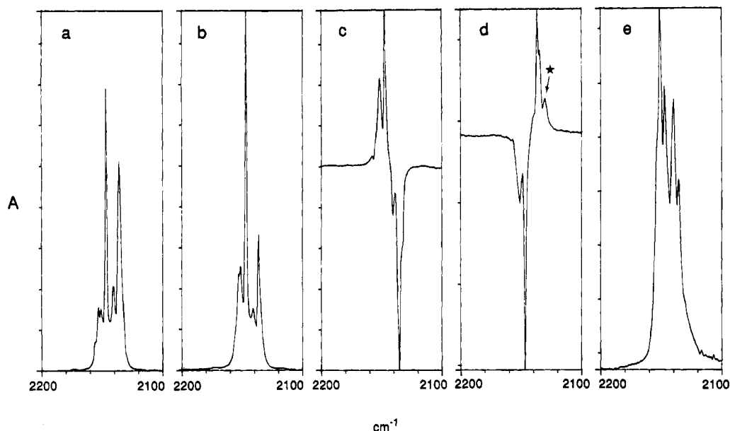
Figure 4. Partial FTIR spectra ( N_2 , 14 K) of s-Z/s-E -acetylketene ( 5 ) produced by FVP ( 400\text{ }^\circ\text{C} , 10^{-6} mbar) of 1 . (a) After deposition; (b) after irradiation at 313 nm for 2 h; (c) difference spectrum (b minus a) ( s-Z-5 top, s-E-5 bottom); (d) difference spectrum after further irradiation with broad-band UV light for 5 min ( s-Z-5 bottom, s-E-5 top); the band at 2130\text{ cm}^{-1} ( \star ) is due to 7 . (e): s-Z/s-E-5 produced by photolysis ( N_2 , 14 K) of 1 at 254 nm for 2 h. For exact values see Table 2.
