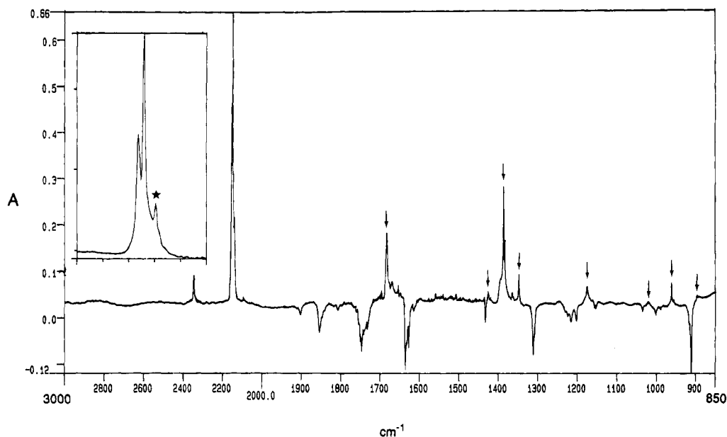
Figure 7. IR difference spectrum (Ar, 14 K) showing the photolysis (366 nm, 4 h) of 2 (bottom) to “photo- Z ”- 5 (top). The inset shows the expanded ketene region (2200–2100 \text{cm}^{-1} ). Bands due to “photo- Z ”- 5 (positive peaks) at 2152, 2149, 1684, 1425, 1387, 1383 (sh), 1348, 1175, 1020, 962, and 897 \text{cm}^{-1} marked by †. The intensity of the band at 1387 \text{cm}^{-1} is significantly diminished by coincidence with a band of 2 at 1388 \text{cm}^{-1} . CO (2139 \text{cm}^{-1} ) marked by ★. The small deviations in frequencies with respect to “photo- Z ”- 5 produced by irradiation of s - Z / s - E - 5 (Figure 6b) are probably due to CO being formed and trapped in the same matrix cavity as “photo- Z ”- 5 . Bands due to 2 (negative peaks) at 1903, 1855, 1748, 1635, 1628, 1435, 1388, 1313, 1218, 1198, 1156, 1024, 999, and 913 \text{cm}^{-1} .
