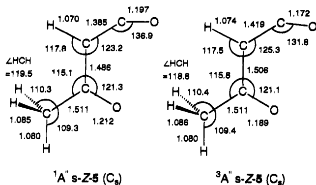
Figure 8. Optimized geometries of the first singlet excited state ( 1A'' , CIS/6-31G ^* ) and the lowest triplet state ( 3A'' , UMP2/6-31G ^* ) of s-Z -acetylketene (bond lengths (Å) and bond angles (deg)).
